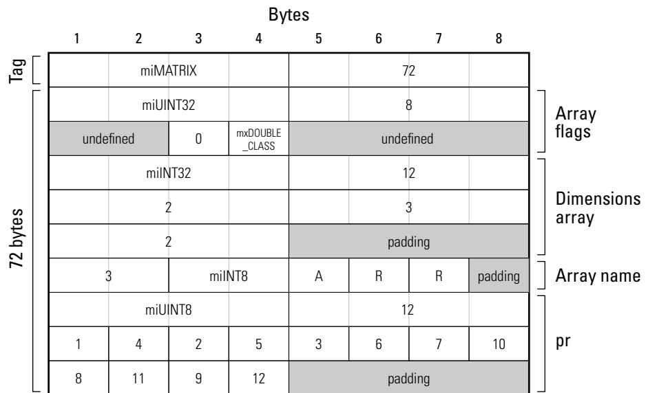
Figure 1-8: Example Numeric Array MAT-file Data Element (Compressed)
