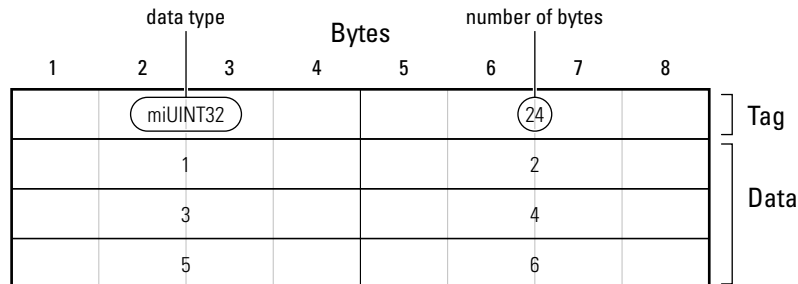
Figure 1-4: Example MAT-File Data Element
