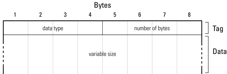
Figure 1-2: MAT-File Data Element Format
