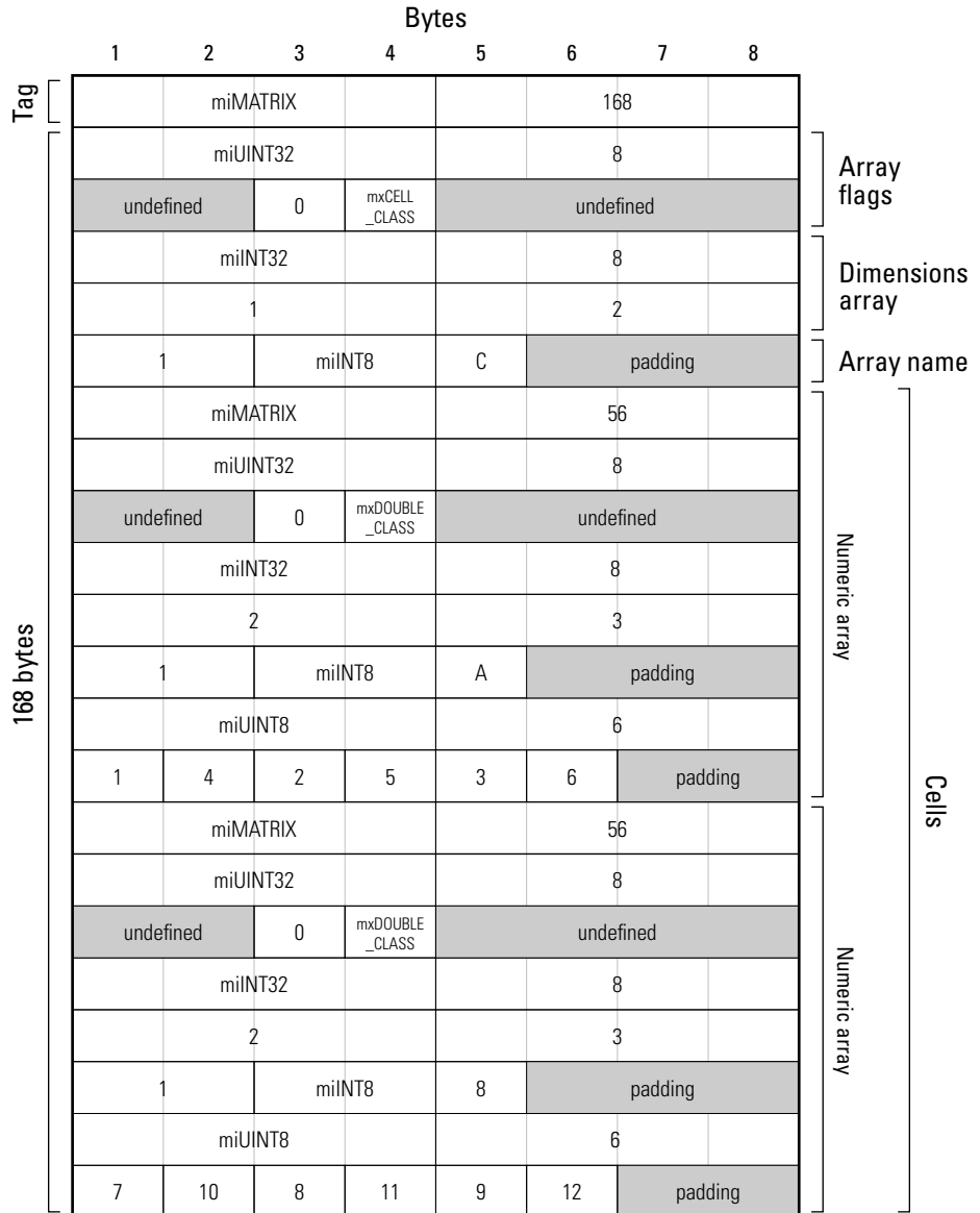
Figure 1-12: Example Cell Array Data Element
