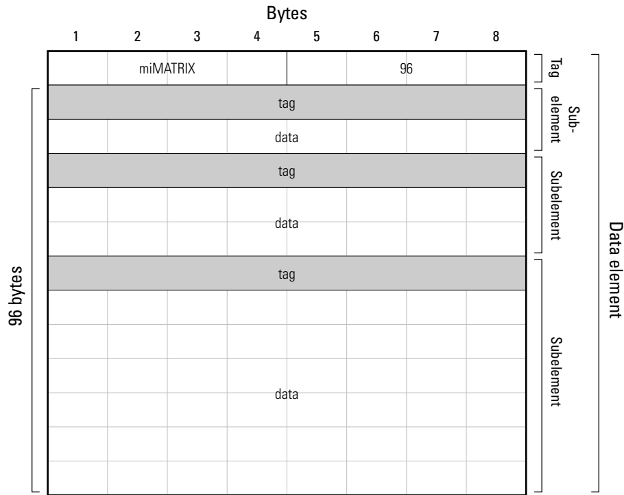
Figure 1-5: MATLAB® Array Data Element with Subelements
