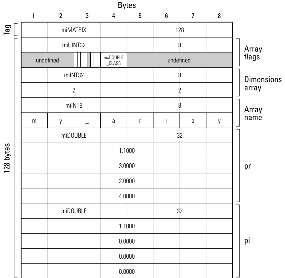
Figure 1-7: Example Numeric Array MAT-File Data Element
