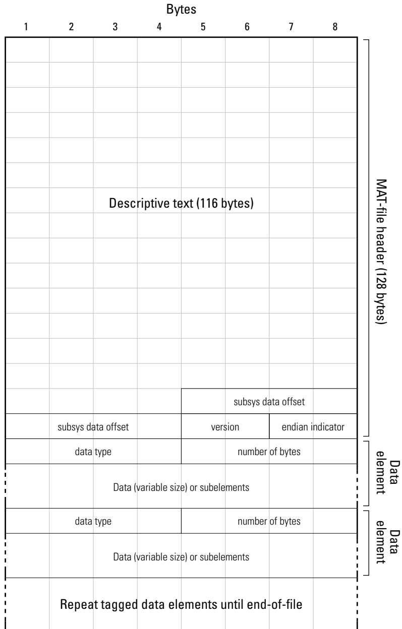
Figure 1-1: MATLAB® Level 5 MAT-File Format
